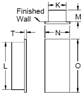
RECESSED
