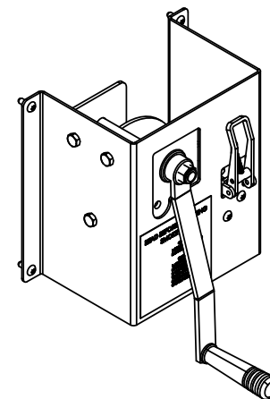
REPLACEMENT PART VIEW (SV-KIT-BRKWINCH)
