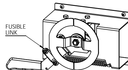
REPLACEMENT PART VIEW (SV-KIT-THERMAL-WINCH)
