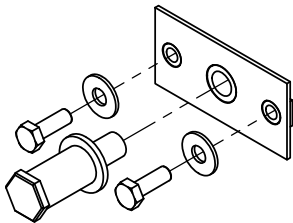
REPLACEMENT VIEW (DOUBLE DOOR ZPS)
