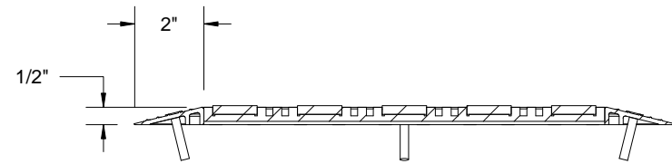
SECTION X-X
