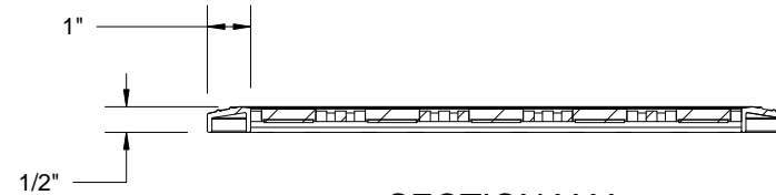
SECTION Y-Y
