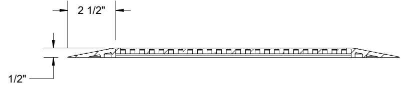
SECTION Y-Y
