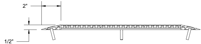
SECTION Y-Y
