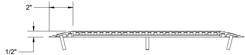
SECTION Y-Y
