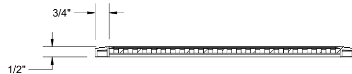
SECTION Y-Y
