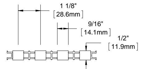
SECTION Y-Y
