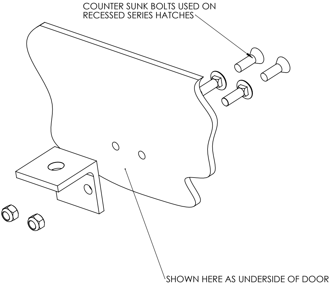
REPLACEMENT PART VIEW
