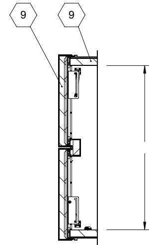
SECTION B-B
