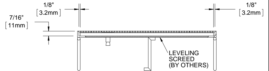
SECTION Y-Y
