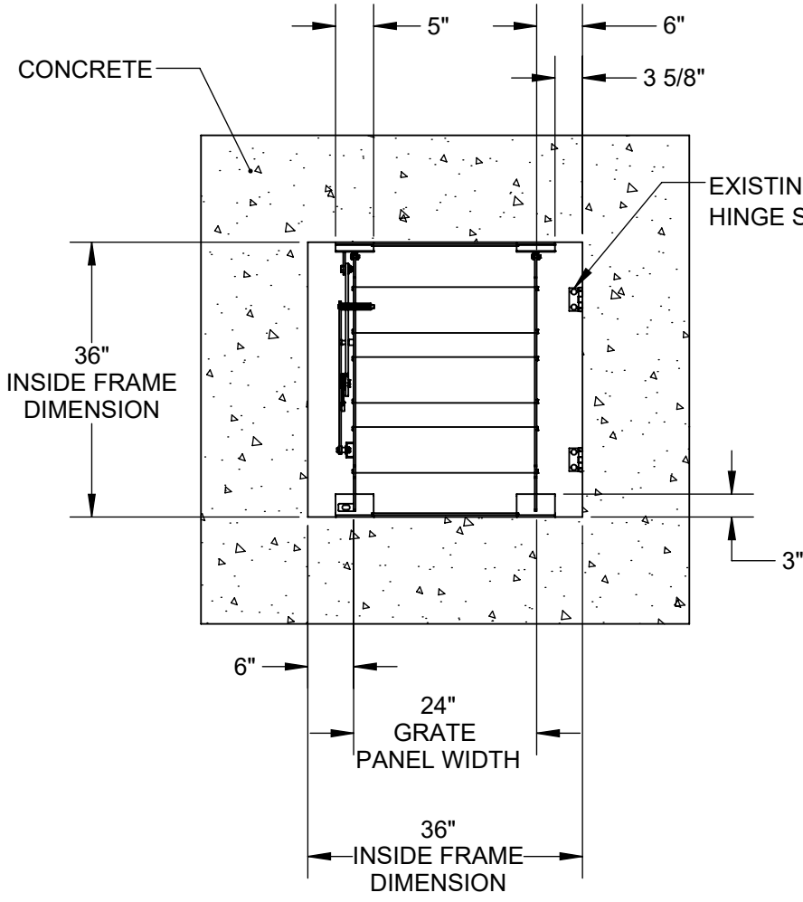
RETROFIT SAFETY GRATE CLOSED
