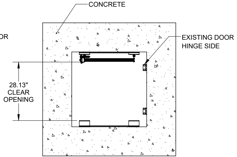
RETROFIT SAFETY GRATE OPEN AND LOCKED IN POSITION
