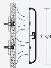
Extended Mount
