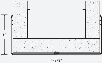
End Wall
