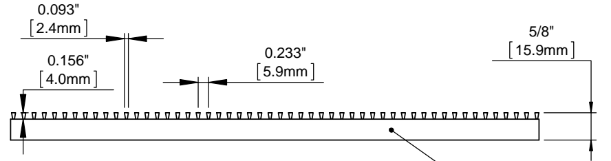
SECTION X GRATE WIDTH
