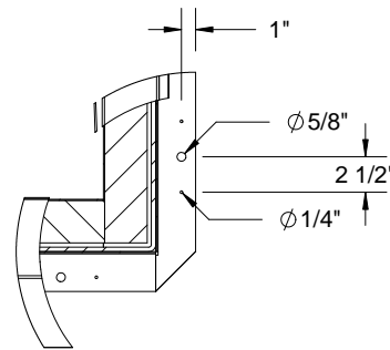
DETAIL G SCALE 1 : 15
