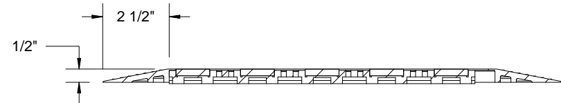
SECTION Y-Y
