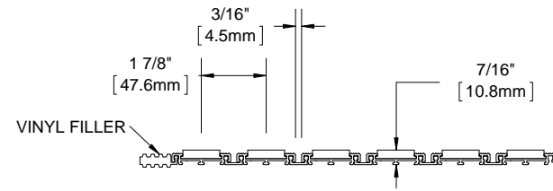
SECTION Y-Y
