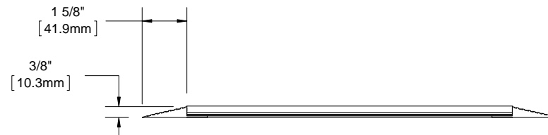
SECTION X-X
