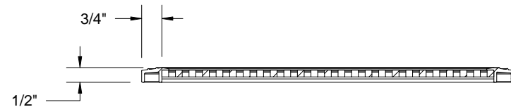
SECTION Y-Y
