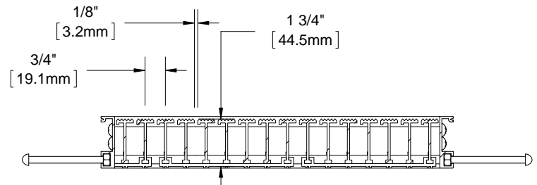
SECTION Y-Y
