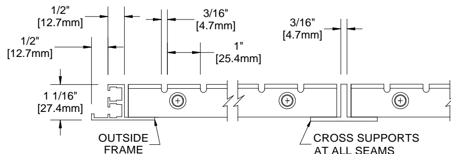
SECTION X-X
