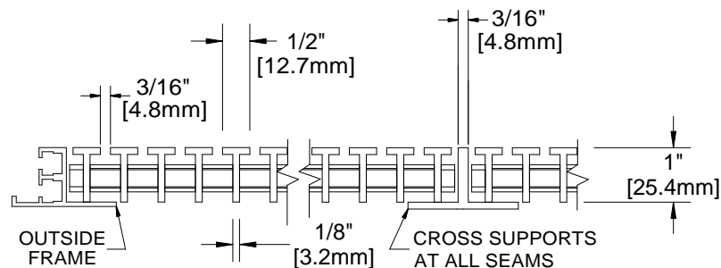
SECTION Y-Y
