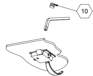
SLAM LATCH DETAIL
